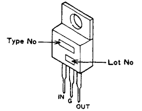
μPC78M12H
